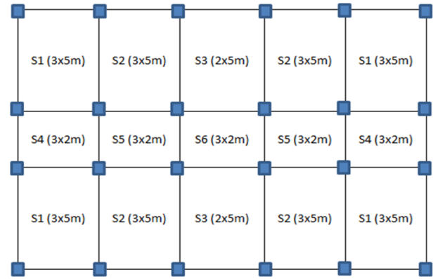
Figure 1: Typical Floor and roof slab layout
