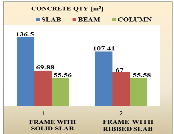
Figure 2: Result of Comparison of Volume of concrete between Slabs, Beams, and Columns
