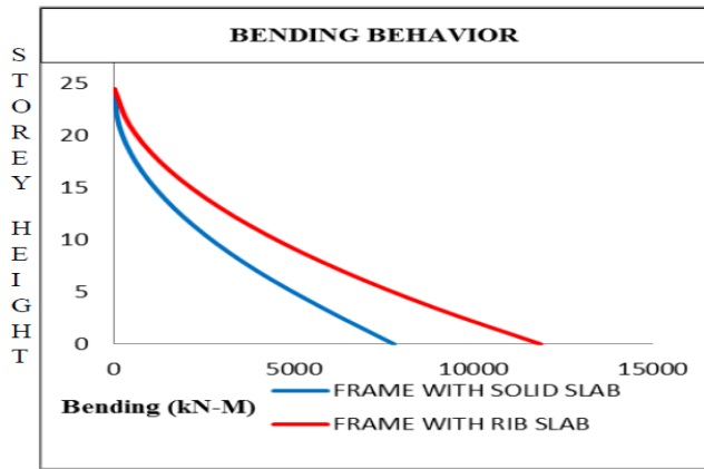
Chart-2: Comparison of Bending Behavior between Frame with Solid Slab and Ribbed Slab
