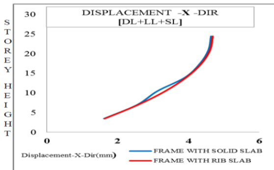
Chart-3: Result of Comparison of displacement -z -dir between Frame with Solid and Ribbed Slab
