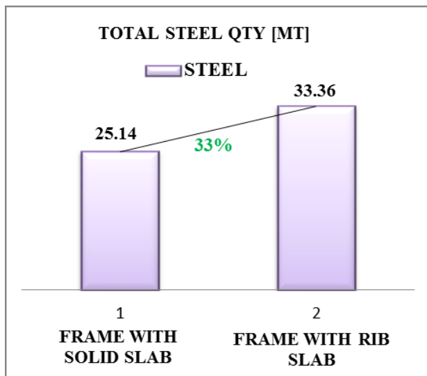
Figure 5 : Result of Comparison of Total quantity of Steel between Frame with Solid and Ribbed Slab
