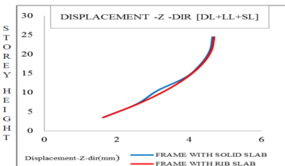
Chart-4: Result of Comparison of displacement -z -dir. between Frame with solid and Ribbed Slab
